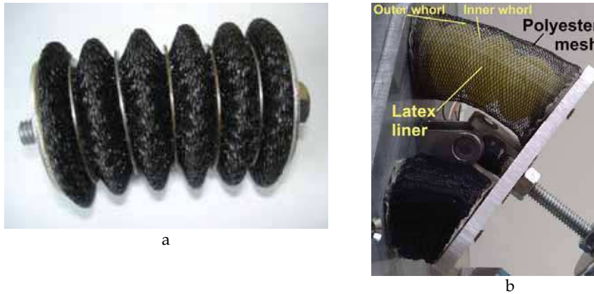
Fig. 14. a - UM-developed rubber bellows used in the OT-8. b - OT-4 bellows comprising a liner and a mesh. We chose yellow latex liner material for this photograph because it contrasts better with the black mesh. However the actual OT-4 bellows have neoprene (black) liners.
