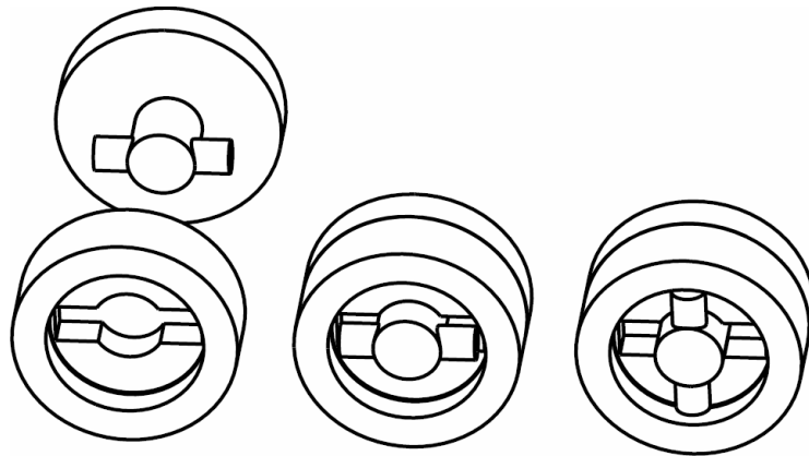
Figure 10. Twist binder : a T-shaped part is inserted in a slotted part, then turned 90 degrees to a press-fit locked position
